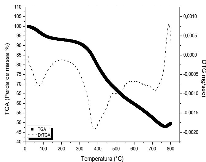
Figura 39: Gráficos da TGA-DTG versus Temperatura do \text{LaNi}_{0,8}\text{Co}_{0,2}\text{O}_3 , 10\text{ }^{\circ}\text{C}.\text{min}^{-1} .
