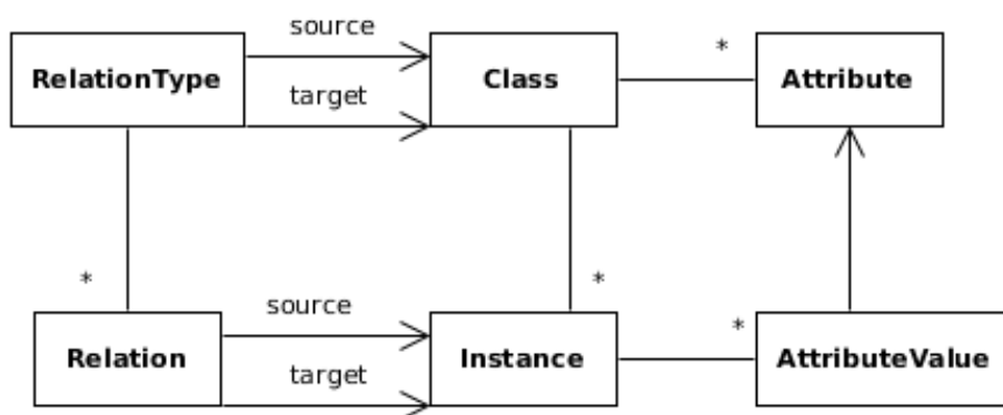
Figura 9 – LOM ( Living Object Model )
