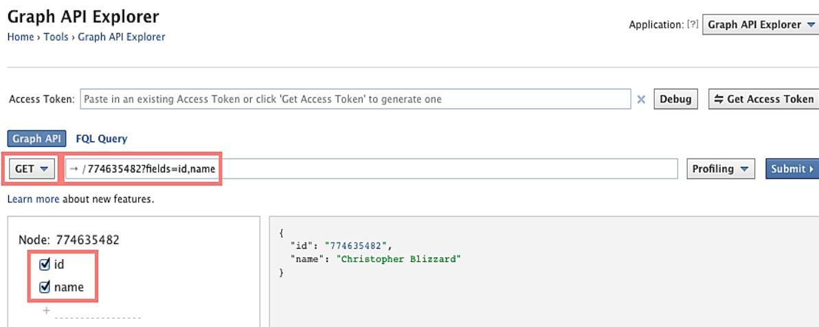
Figura 6 - Graph API Explorer
