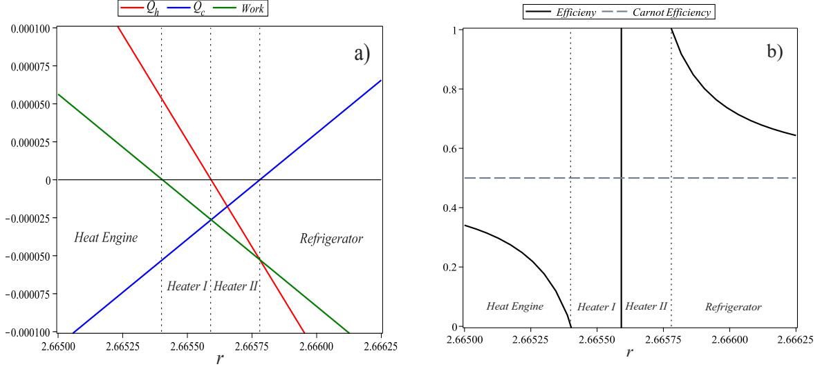
Figure 4.8 In (a) we have the work done W (green), the heat absorbed Q_h (red) and released Q_c (blue) against the compression ratio r : the observed behaviour reminds us something like a phase transition. In (b), the efficiency \eta (solid curve) and the Carnot efficiency \eta_c (dashed horizontal curve) against the compression ratio r are depicted: it is observed a drastic fall intersecting the r -axis and continuing to negative values till Q_h goes to zero, where the efficiency explodes to infinity. We keep the same values, as usual, V_h = 10, \Delta_1 = 10, \Delta_2 = 3, kT_h = 2, kT_c = 1 . The values of Q_h , Q_c and W are given in units of \mu\text{eV} .
