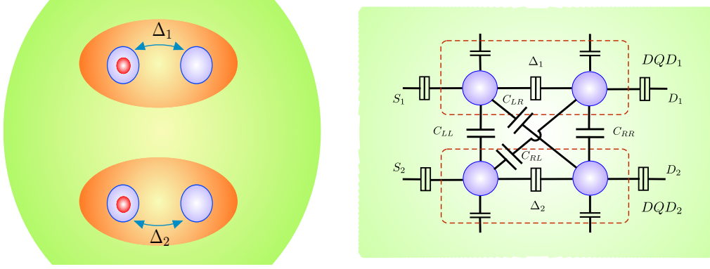
Figure 4.1 The left picture shows a schematic representation of the physical model with two coupled DQDs. The purple spheres represent the quantum dots, the electrons are represented by the smaller red spheres inside the quantum dots and \Delta_{1,2} stands for the tunneling coupling of the DQD_{1,2} . The right picture is the equivalent circuit diagram of the device. Tunnel couplings are represented by two bars as in \Delta_1 and \Delta_2 , S_{1,2} and D_{1,2} are, respectively, the source and drain of the DQD_{1,2} , and the capacitors C_{LL} , C_{RR} , C_{LR} and C_{RL} connect the DQDs.
