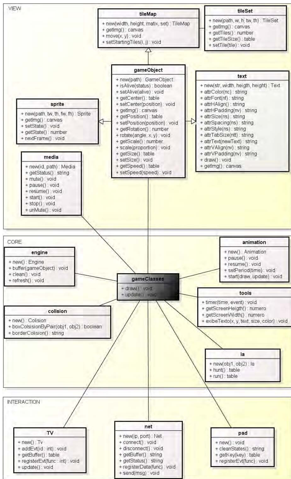
Figura 15 – Diagrama de Classes do framework Athus
