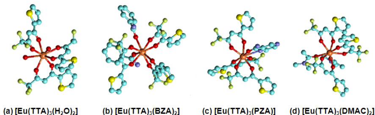
Figura 6 – Exemplos de complexos \beta -dicetonatos de lantanídeos: (a) [\text{Eu}(\text{TTA})_3(\text{H}_2\text{O})_2] , (b) [\text{Eu}(\text{TTA})_3(\text{BZA})_2] , (c) [\text{Eu}(\text{TTA})_3(\text{PZA})] , (d) [\text{Eu}(\text{TTA})_3(\text{DMAC})_2] 34 .
