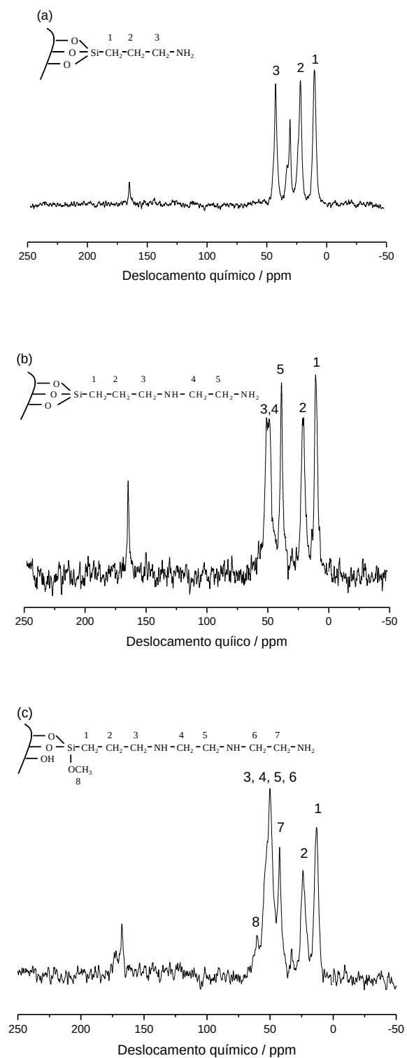
Figura 5.11 - Espectros de RMN de ^{13}\text{C} para as amostras HMS-1N (a), HMS-2N (b) e HMS-3N (c).
