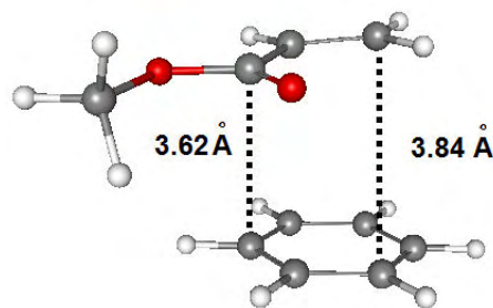
Figure 4. Optimized geometry of the benzene...methyl-acrylate complex 4 using MPW1B95/6-311++G(2d,2p) 6d level of theory.
