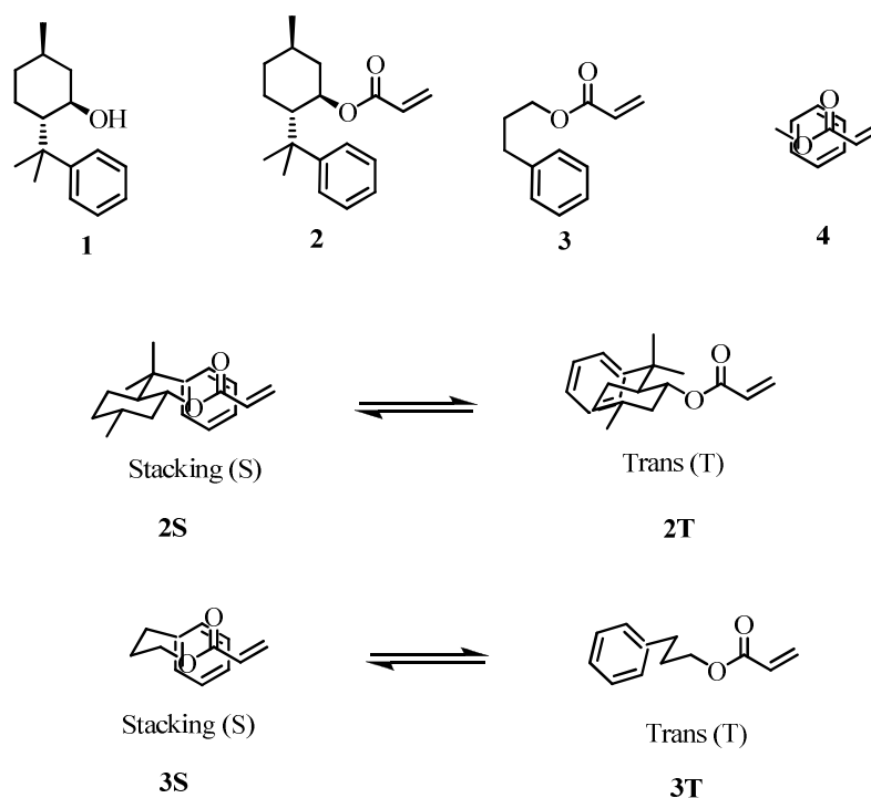
Figure 1. Structures for calculated conformations.
