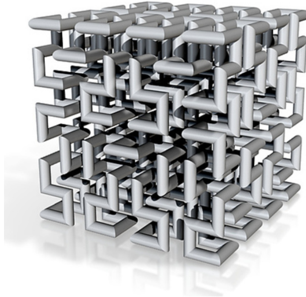
Figure 3.1: Sketch of an iteration of a tridimensional space-filling curve.
