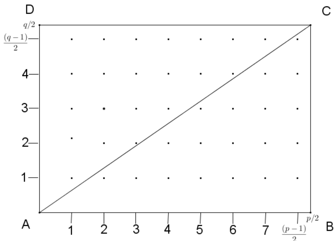
Figura 2.1: y = \frac{q}{p}x
