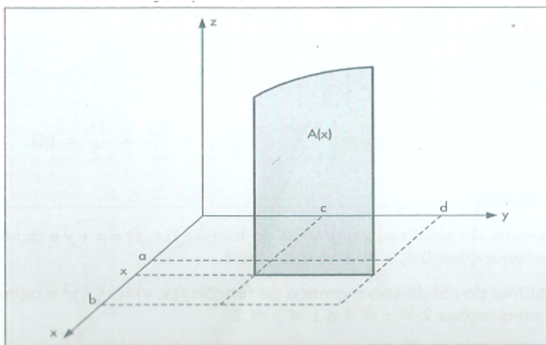
Figura 4.2: Integral Parcial A(x)
