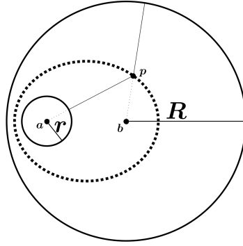
Figura 3.6: Elipse
