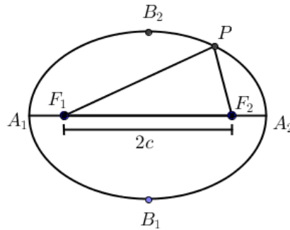
Figura 4.18: Elipse
