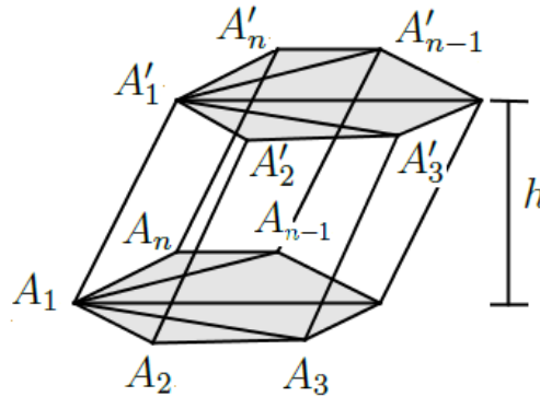
Figura 2.29: Prisma qualquer.
